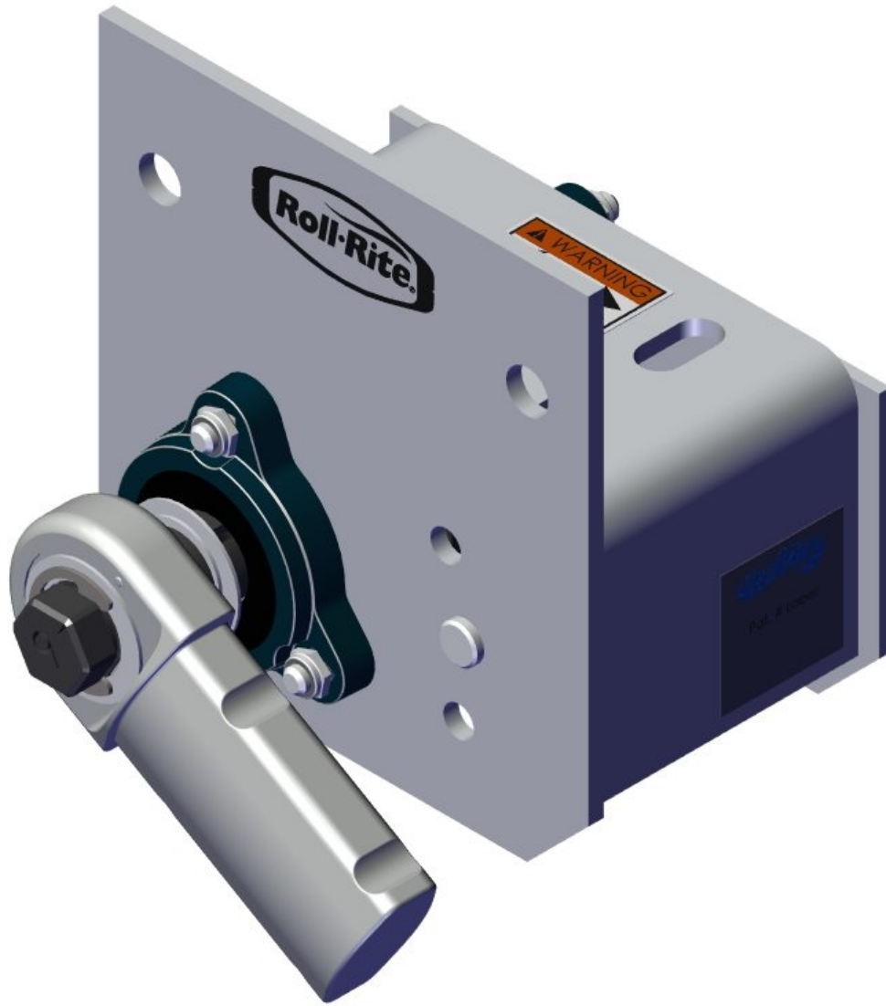
Pivot. UB Assembly 4-Spr UB Pivot w/o Tube - Driver
