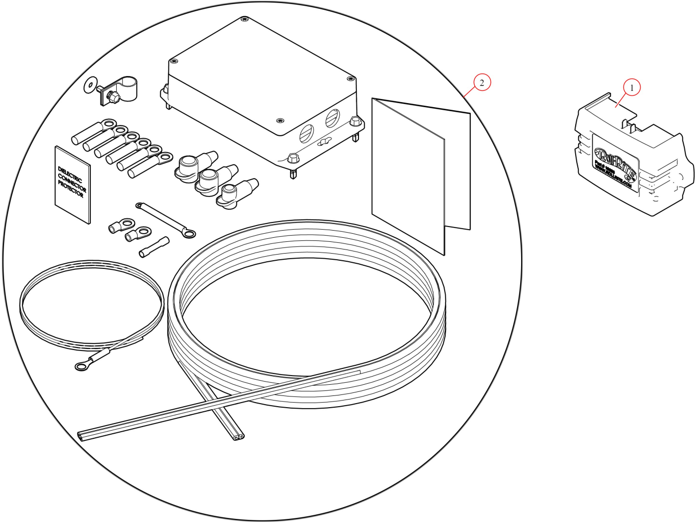
104148 Smart Breaker & enclosure with 10695 relay and 8ga terminals
