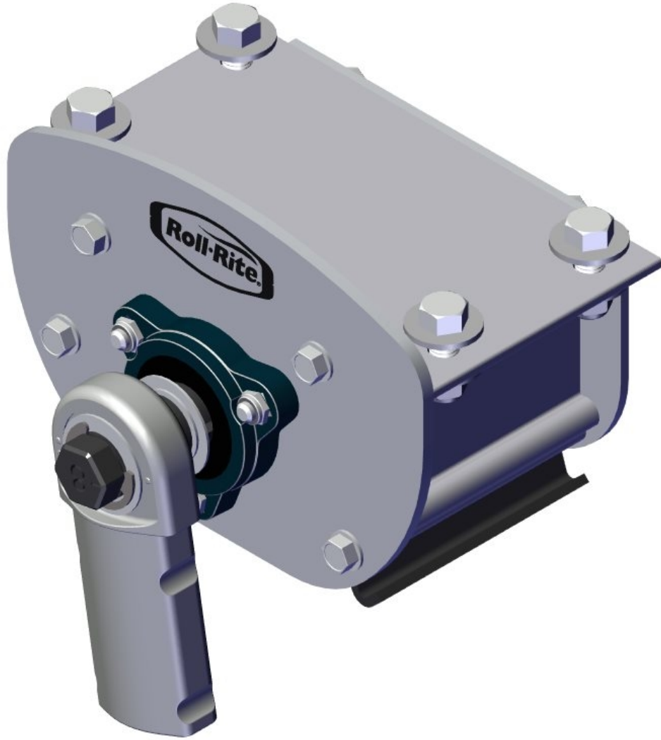
Pivot. UB Assembled STS 8-Spr Front
